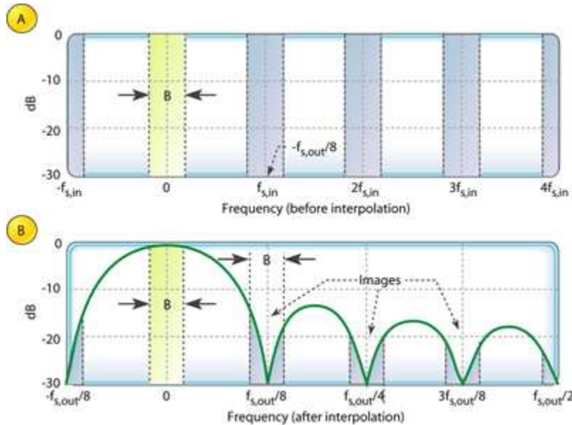
Figure 7: 1st-order, D = R = 8 , interpolating CIC filter spectra: input spectrum; output spectral images
