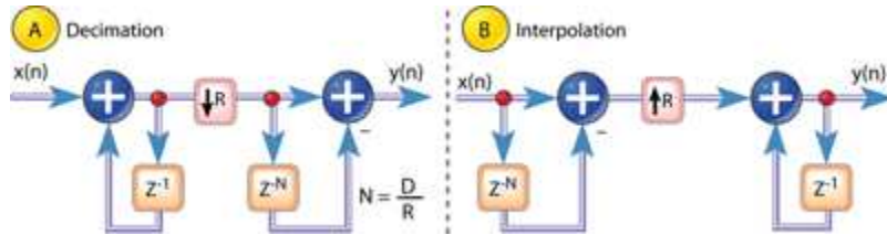
Figure 9: Single-stage CIC filter implementations: for decimation; for interpolation
