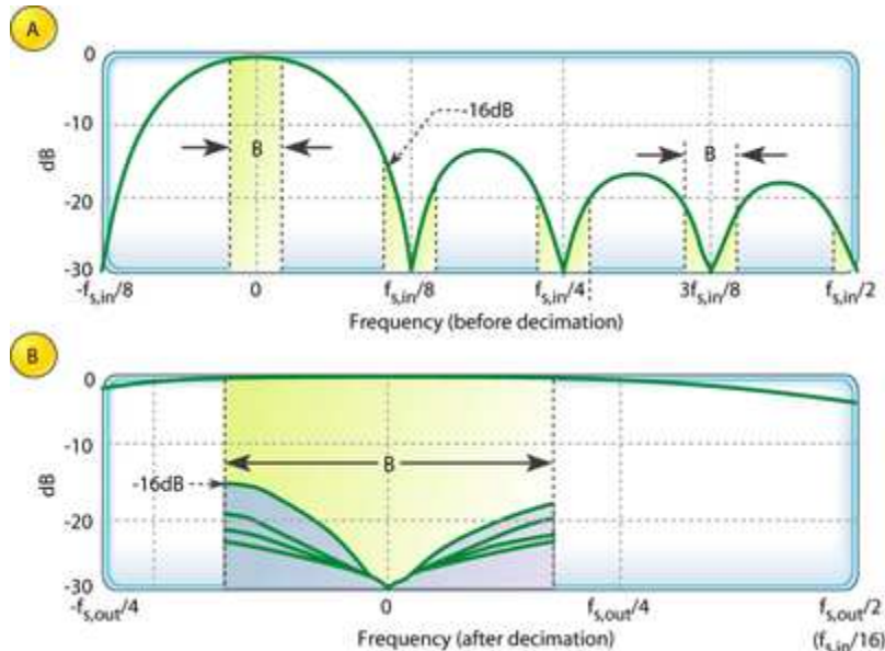
Figure 6: Magnitude response of a 1st-order, D = 8 , decimating CIC filter: before decimation; aliasing after R = 8 decimation
