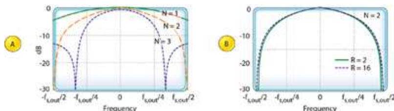
Figure 10: CIC decimation filter responses: for various values of differential delay N , when R = 8 ; for two decimation factors when N = 2
