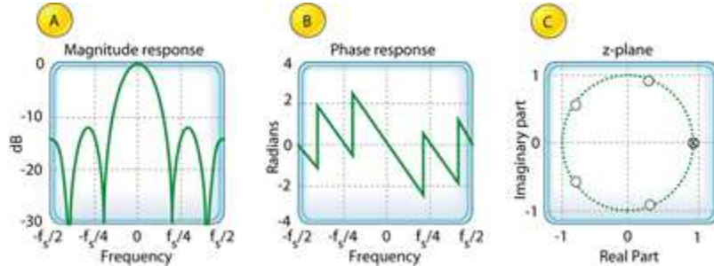
Figure 4: Characteristics of a single-stage CIC filter when D = 5
