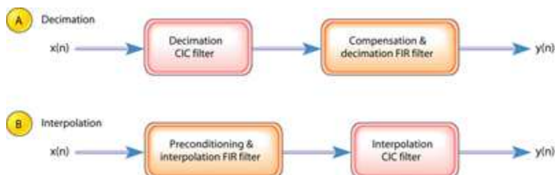
Figure 1: CIC filter applications
