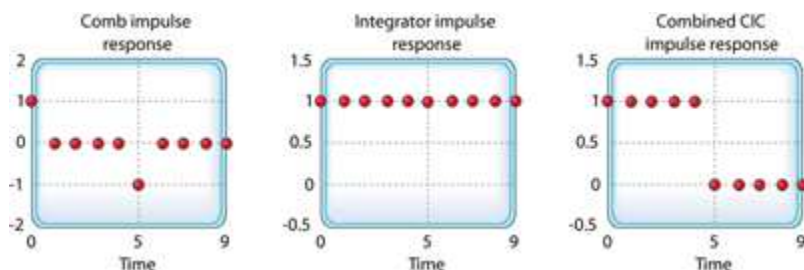
Figure 3: Single-stage CIC filter time-domain responses when D = 5
