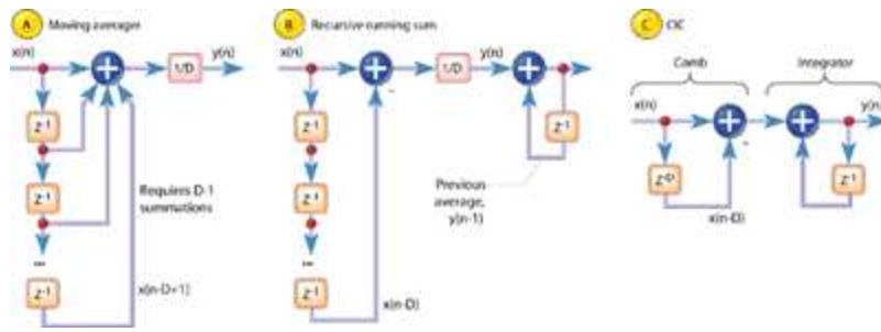
Figure 2: D-point averaging filters
