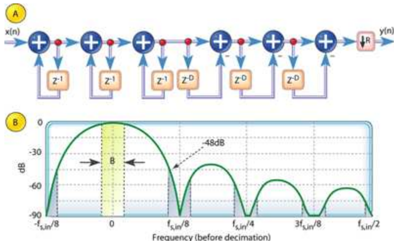
Figure 8: 3rd-order CIC decimation filter structure, and magnitude response before decimation when D = R = 8
